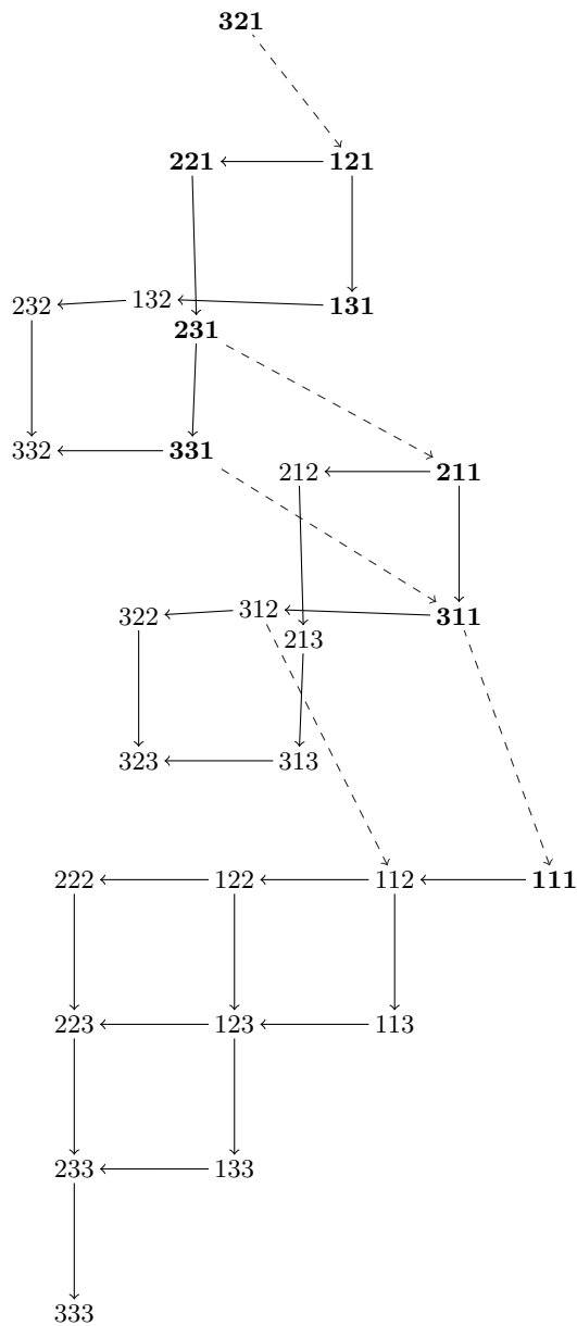
FIGURE 5. The tensor product of KR crystals \mathcal{B}^\mu = B^{1,1} \otimes B^{1,1} \otimes B^{1,1} , which is also the DARK crystal \mathcal{B}^{\mu;\mathbf{w}} for \mu = (1, 1, 1) and \mathbf{w} = (s_2s_1, s_2s_1, s_2s_1) . Its charge weighted character is the modified Hall-Littlewood polynomial H_{111}(\mathbf{x}; q) = s_{111} + (q + q^2)s_{21} + q^3s_3 = \kappa_{111} + (q + q^2)\kappa_{012} + q^3\kappa_{003} . Horizontal and vertical arrows give the \tilde{f}_1, \tilde{f}_2 edges, respectively. The dashed arrows are the \tilde{f}_0 -edges of \mathcal{B}^\mu \otimes B(\Lambda_0) which have both ends in \mathcal{B}^{\mu;\mathbf{w}} \otimes u_{\Lambda_0} \subset \mathcal{B}^\mu \otimes B(\Lambda_0) . Since \mu is constant, the corresponding generalized Demazure crystal \text{AGD}(\mu; \mathbf{w}) = \Theta_\mu(\mathcal{B}^{\mu;\mathbf{w}} \otimes u_{\Lambda_0}) (via Theorem 2.11) is an actual affine Demazure crystal, namely \mathcal{F}_{s_2s_1\tau s_2s_1\tau s_2s_1}\{u_{\Lambda_1}\} \subset B(\Lambda_0) .
