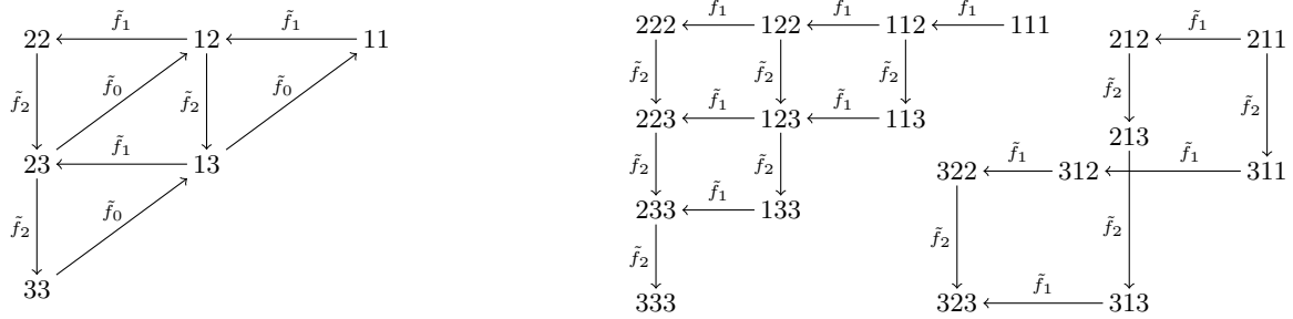
FIGURE 3. For \ell = 3 , the KR crystal B^{1,2} (left) and \text{Res}_{\mathfrak{sl}_\ell} \mathcal{B}^{(2,1)} = \text{Res}_{\mathfrak{sl}_\ell} B^{1,1} \otimes B^{1,2} (right).
